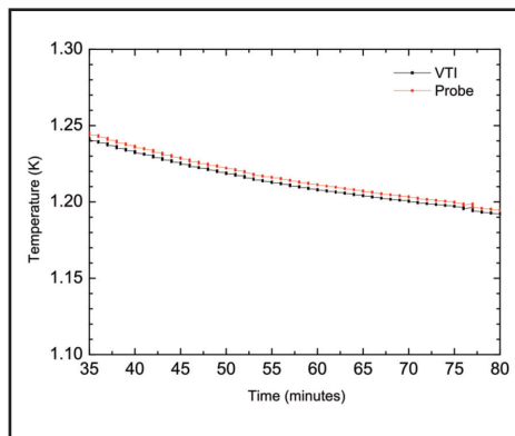
VTI Base Temperature (Liquid Column)
