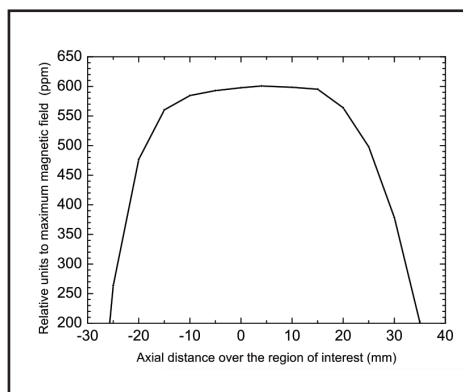
Magnetic Field Axial Profile of the 10.1 T magnet
