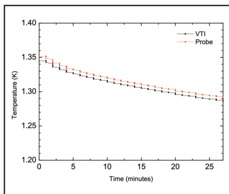
VTI Base Temperature (Continuous Flow)
